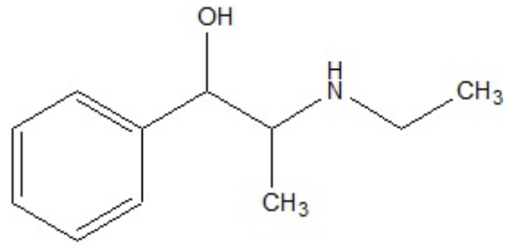
N-ethynorephedrine
